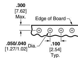
Recommended Mounting Hole Pattern for .300 [7.62] Max. Edge of Board (Solder Side of Board Shown)
