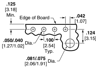
Recommended Mounting Hole Pattern for .125 [3.18] Min. Edge of Board (Solder Side of Board Shown)
